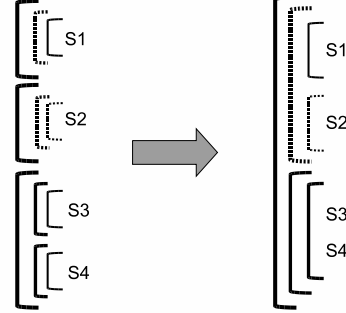
Figure 2: Controllable multi-level loop fusion.
